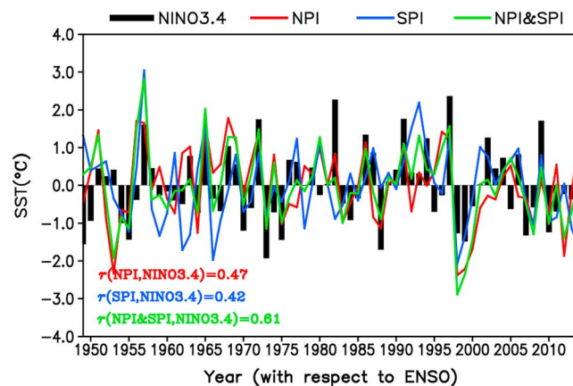
Figure 8. Time series of the observed boreal winter Niño3.4 index (black bars), and the cross-validated hindcasts of the boreal winter Niño3.4 index generated by empirical model (1) using both the combined NPI and SPI (green line), using the NPI alone (red line) and using the SPI alone (blue line). The correlations between various time series are given in the bottom left corner.
