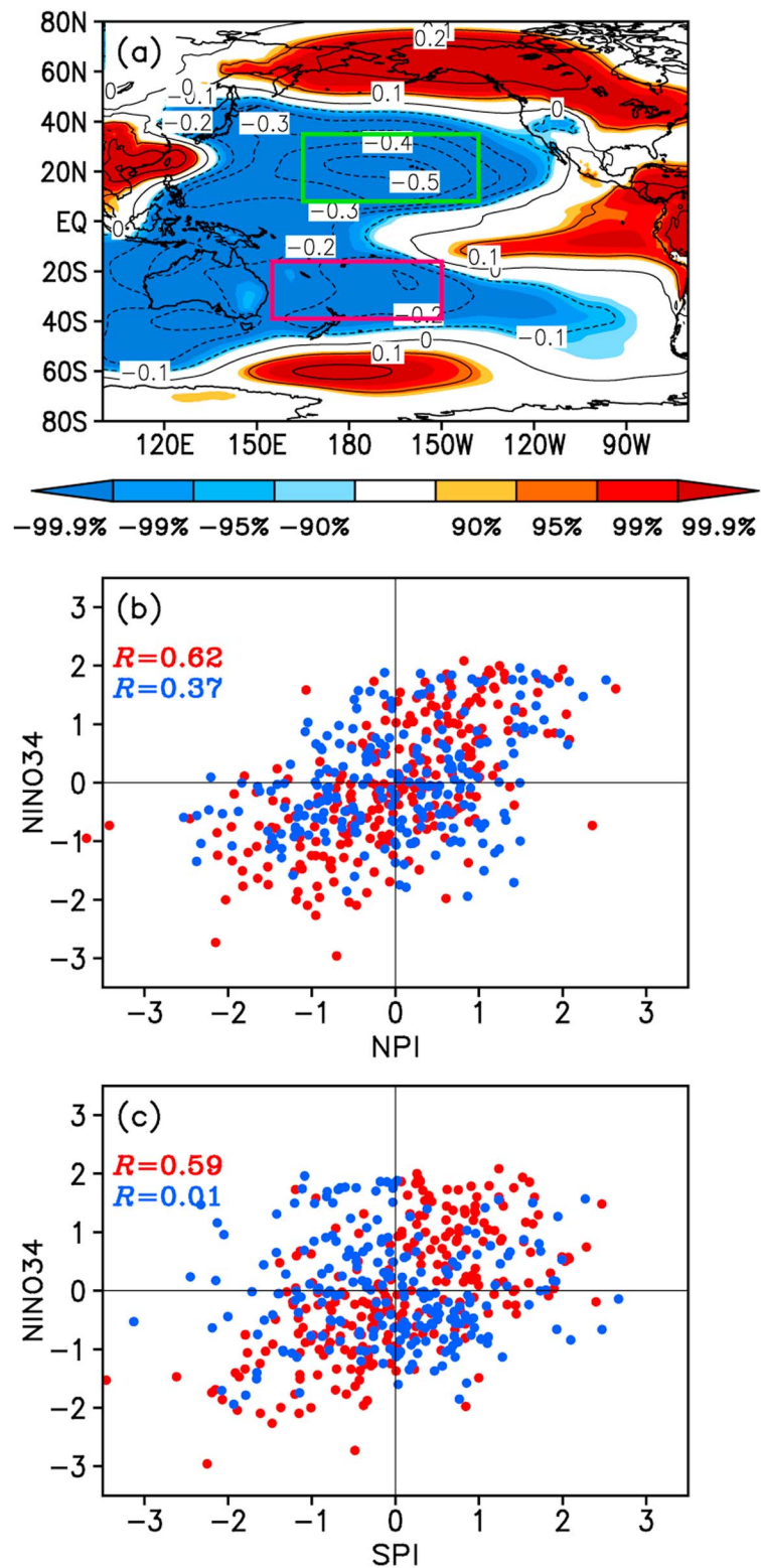
Figure 11. (a) Correlation maps between the boreal winter (NDJFM) SLP anomalies and the Niño3.4 index a year later in the 501 year piControl experiment of CESM. Areas with a correlation significant at or above the 90% confidence level are shaded. The green box (165°E–138°W, 8°–35°N) is used to define the NPI, and the magenta box (155°E–150°W, 39°–16°S) is used to define the SPI. (b) Scatterplots of the boreal winter NPI versus the Niño3.4 index a year later. Red (blue) circles indicate the years in which the NPI has the same (opposite) sign as the SPI. (c) As in 11b but for scatterplots of the boreal winter SPI versus the Niño3.4 index a year later.
