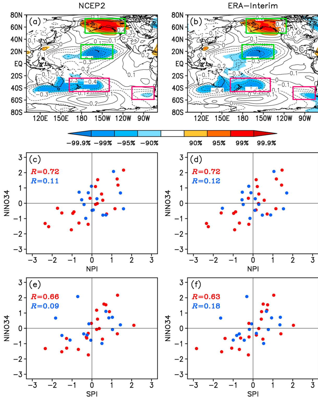
Figure 5. (a) Correlation map of the boreal winter (NDJFM) Niño3.4 index with the previous boreal winter SLP anomalies based on the NCEP2 data set. Areas with a correlation significant at or above the 90% confidence level are shaded. The two green boxes ( 175^{\circ}\text{E} – 117^{\circ}\text{W} , 50^{\circ} – 74^{\circ}\text{N} and 179^{\circ}\text{E} – 135^{\circ}\text{W} , 8^{\circ} – 31^{\circ}\text{N} ) are used to define the NPI, and the magenta box ( 155^{\circ}\text{E} – 150^{\circ}\text{W} , 46^{\circ} – 24^{\circ}\text{S} ) is used to define the SPI. (c) Scatterplots of the boreal winter NPI versus the Niño3.4 index a year later. Red (blue) circles indicate the years in which the NPI has the same (opposite) sign as the SPI. Both the NPI and SPI are calculated from the NCEP2 data set. (e) As in Figure 5c but for scatterplots of the boreal winter SPI versus the Niño3.4 index a year later. (b, d, and f) As in Figures 5a, 5c, and 5e, respectively, but for ERA-Interim.
